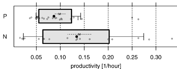
Fig. 6. \frac{1}{t_{work}} : Productivity measured as the inverse of total working time (number of programs per hour, one could say).
