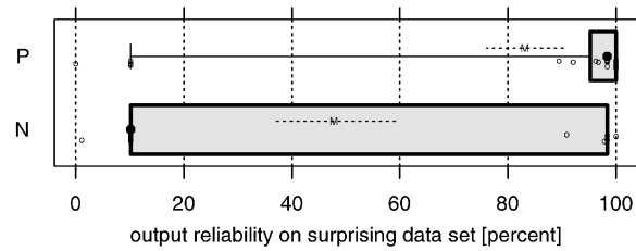
Fig. 2. Output reliability for the data set with possible no digit in a phone number.
