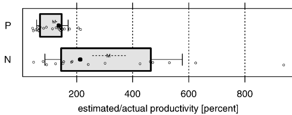
Fig. 5. \frac{prod_{estim}}{prod_{actual}} : Quotient of estimated and actual productivity, each measured in lines of code per hour.
