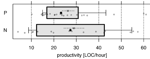
Fig. 7. \frac{LOC}{t_{work}} : Productivity measured as the number of statement LOC written per hour.
