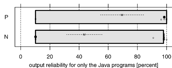
Fig. 3. Output reliability for the data set with possibly no digits in a phone number, measured only for the Java programs.
