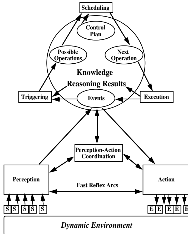
Figure 2. The Agent Architecture.
